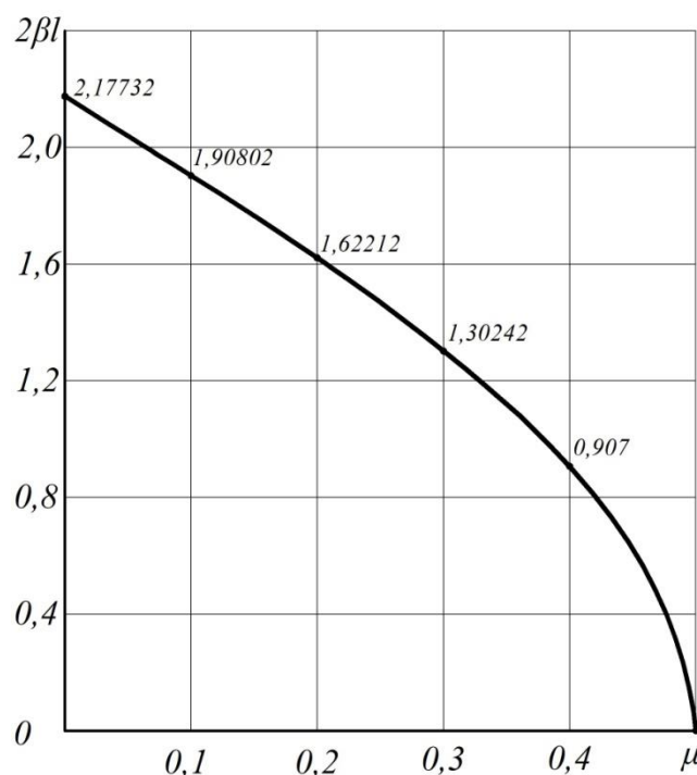
Figure 4. Graphical representation of functions for solving equations (45)
